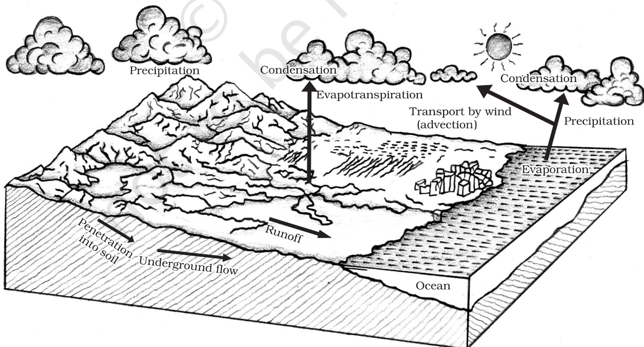
Figure 13.1 : Hydrological Cycle
